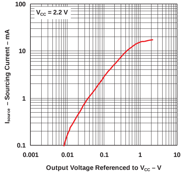
SOURCING CURRENT vs OUTPUT VOLTAGE
