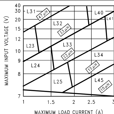
Figure 7-3. LM2676-5
