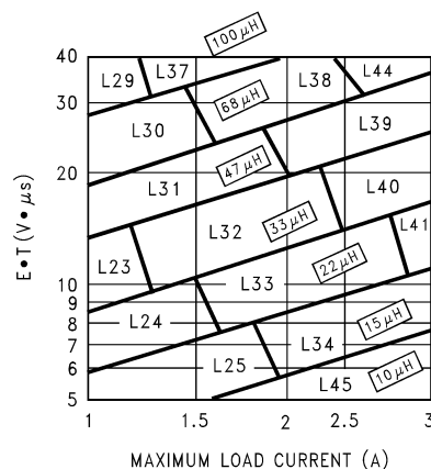
Figure 7-5. LM2676-ADJ
