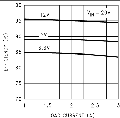
Figure 5-4. Efficiency versus I_{LOAD}
