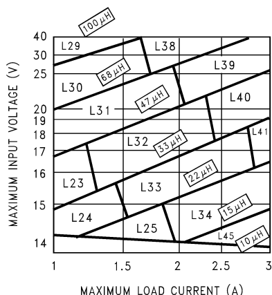
Figure 7-4. LM2676-12
