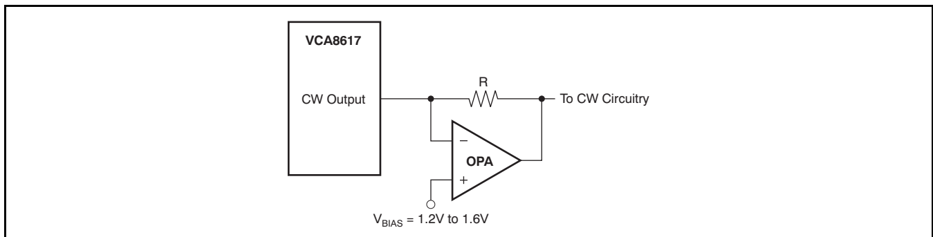
Figure 63. Operational Amplifier
