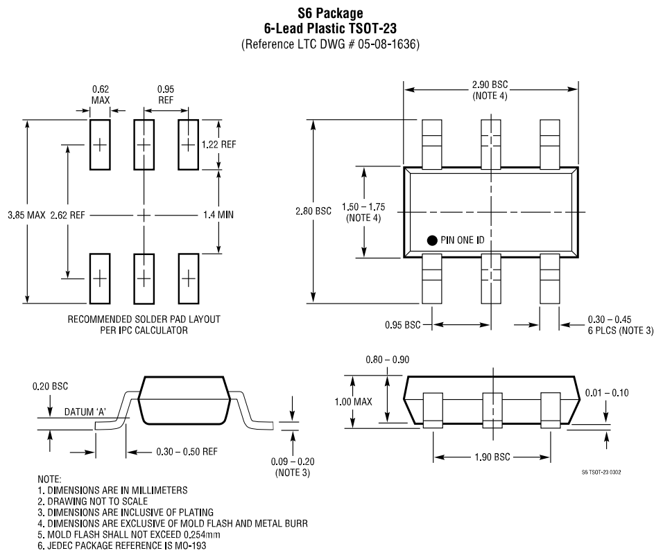
Figure 28. Package Drawing
