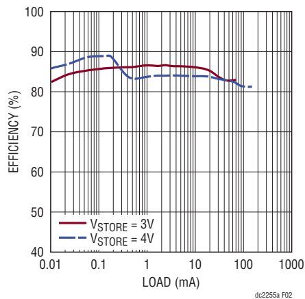
Figure 2. DC2255A Efficiency vs Load with Part Running from V_{STORE} Input. V_{OUT} = 3.3V
