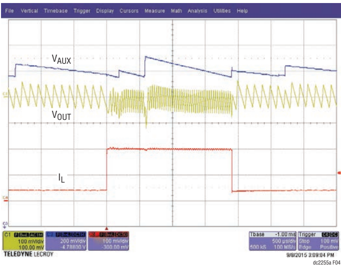
Figure 4. DC2255A Load Step Response. V_{IN} = 3V , V_{OUT} = 3.3V , Load Step is from 40mA to 200mA
