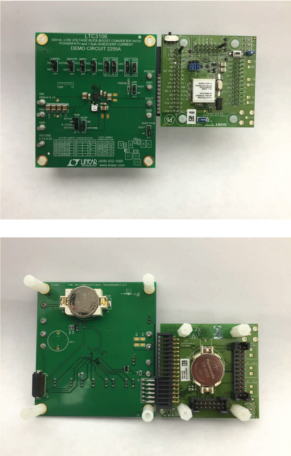
Figure 7. DC2255A Top and Bottom View of DC2255A Connected to Dust Mote.
