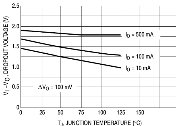
Figure 2. Dropout Voltage vs. Junction Temperature
