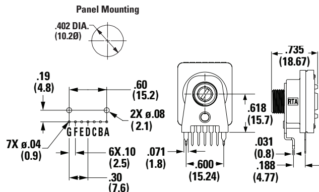
B M10 x 0.75 Metric Threaded Bushing With Bracket
