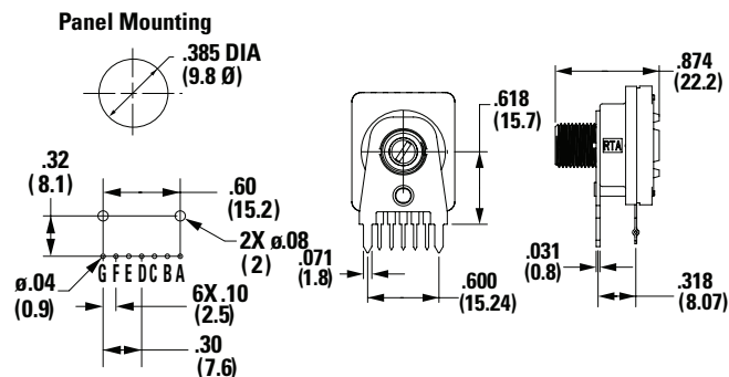
C 3/8-32 Threaded Bushing With Straight Bracket
