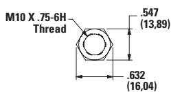
Part No. 205D00201CH Metric
