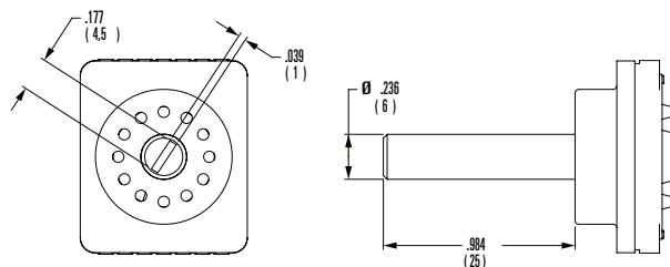
FLS Flush Shaft With Screwdriver Slot and Position Indicator
