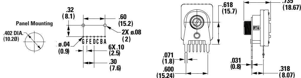
D M10 x 0.75 Metric Threaded Bushing With Straight Bracket
