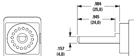
25F 0.984 (25.0) Shaft with Flat
