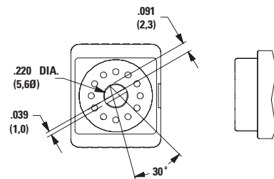
FLS Flush Shaft With Screwdriver Slot and Position Indicator
