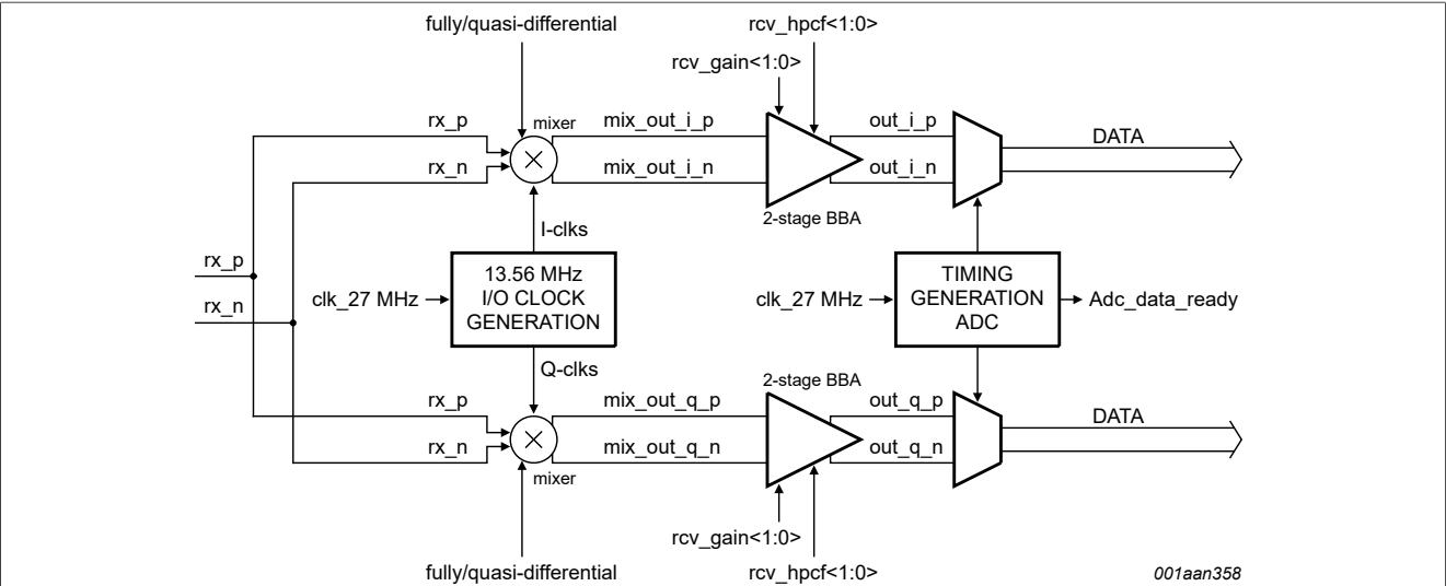
Figure 24. Block diagram of receiver circuitry
