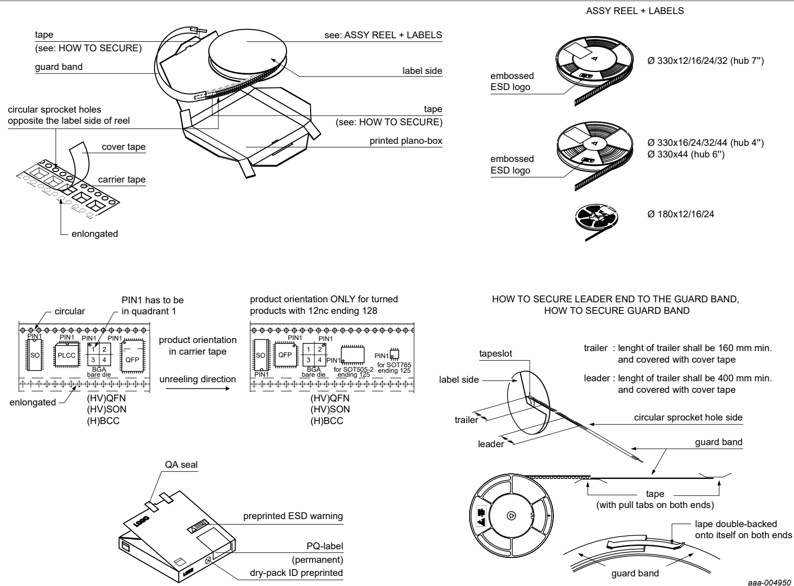
Figure 37. Packing information Reel
