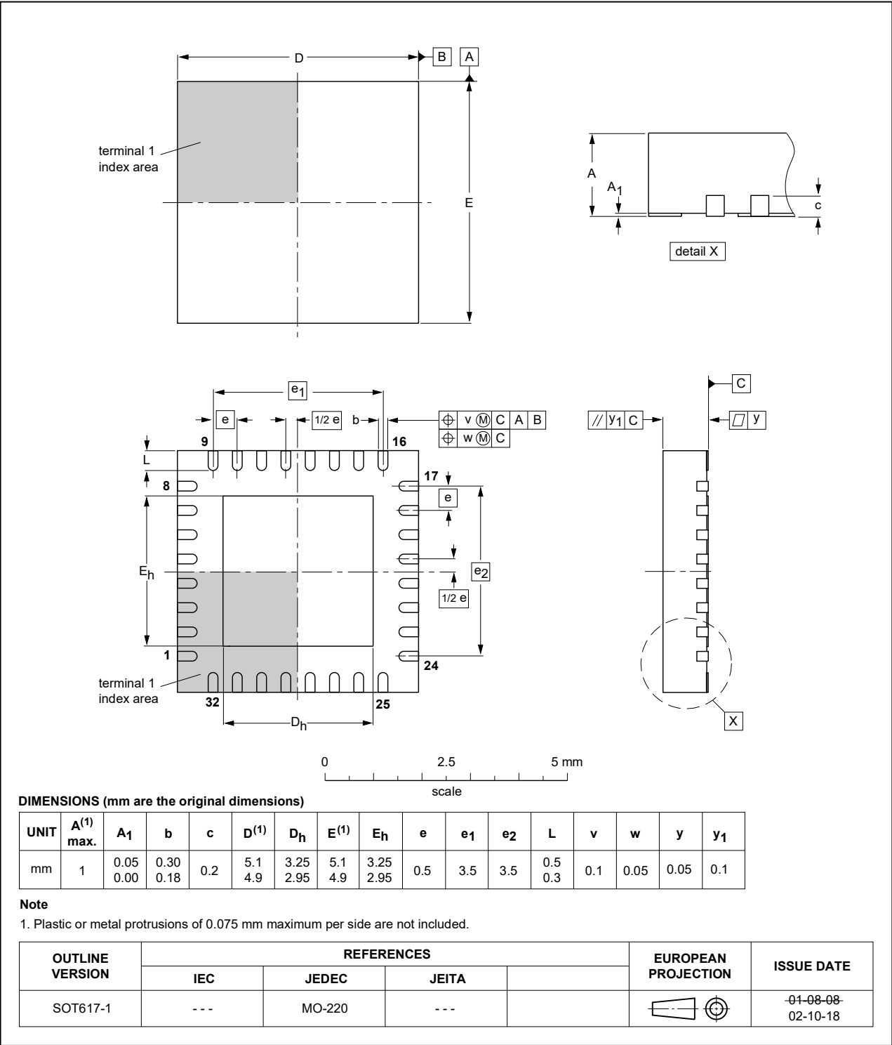
Figure 33. Package outline SOT-617-1 (HVQFN32)
