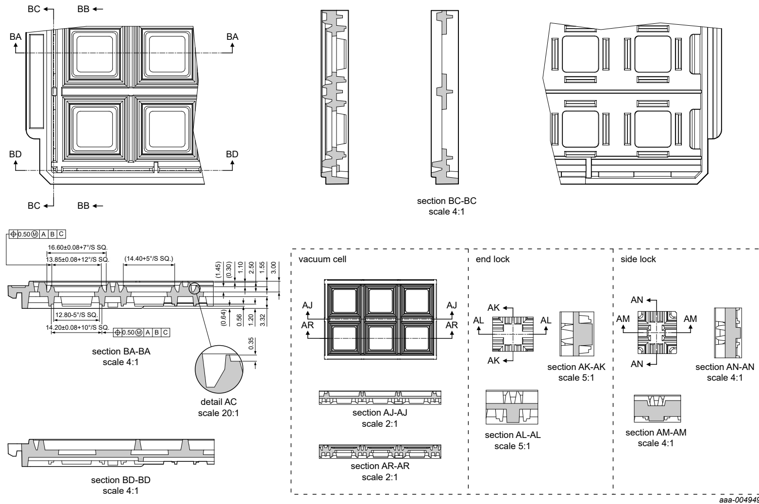
Figure 36. Tray details
