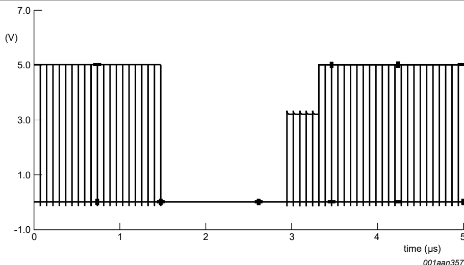
Figure 23. Example 2: overshoot_t1 = 0d; overshoot_t2 = 5d
