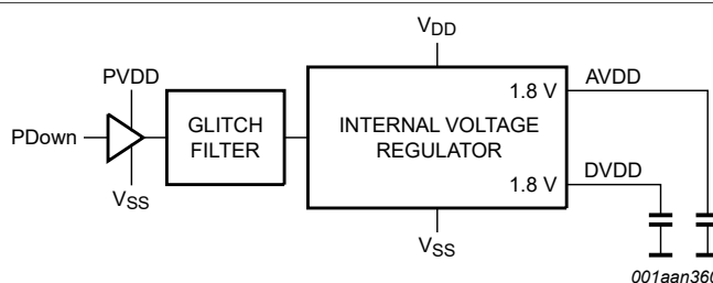
Figure 29. Internal PDown to voltage regulator logic
