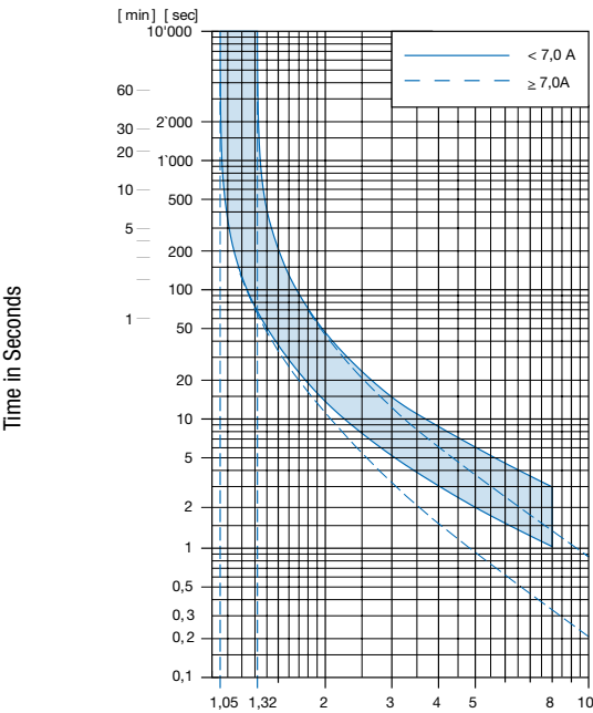
Time-Current-Curves
