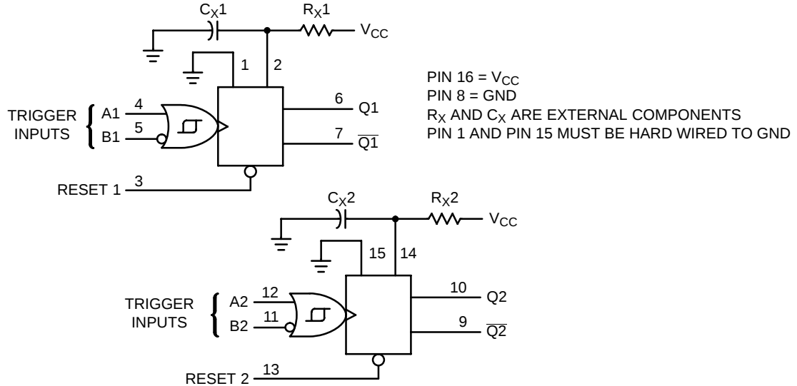
Figure 2. Logic Diagram
