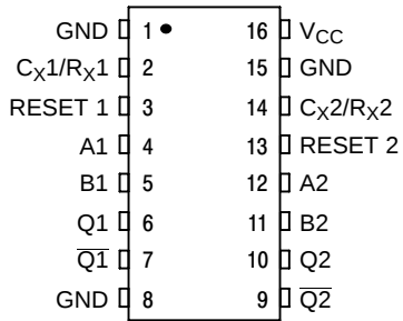
Figure 1. Pin Assignment
