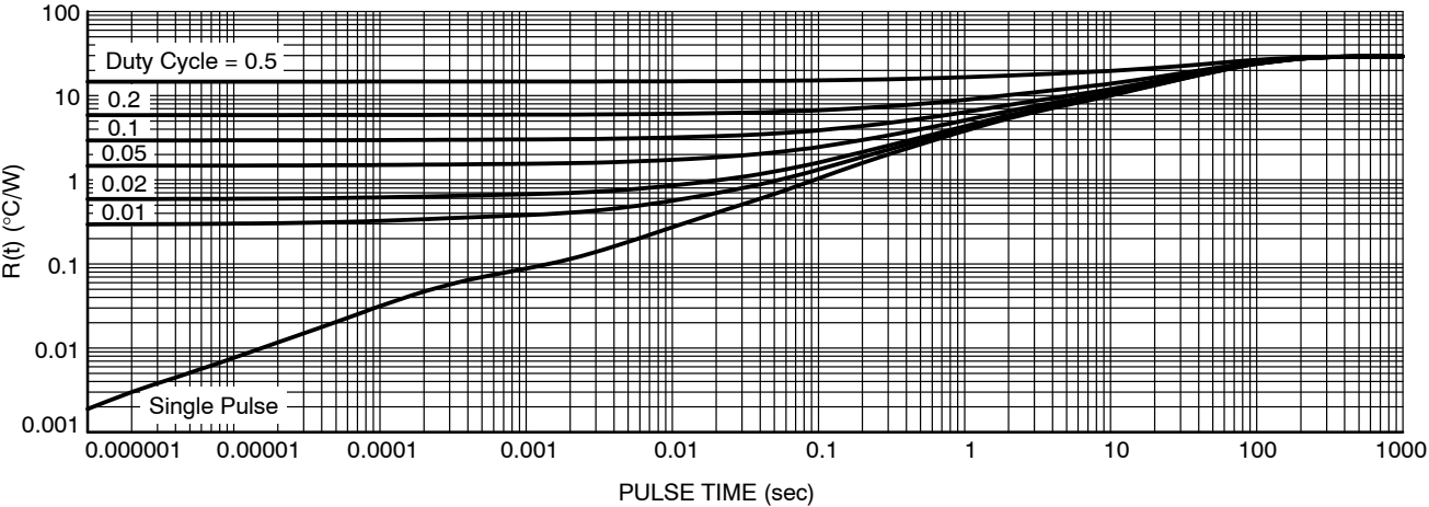
Figure 13. Thermal Characteristics
