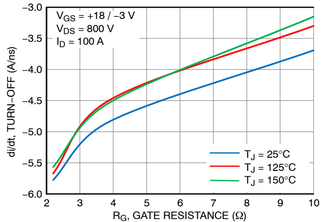
Figure 20. \frac{di}{dt} Turn OFF vs. Gate Resistance V_{DS} = 800 V
