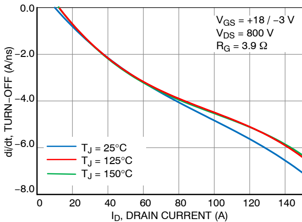
Figure 19. \frac{di}{dt} Turn OFF vs. Drain Current V_{DS} = 800 V
