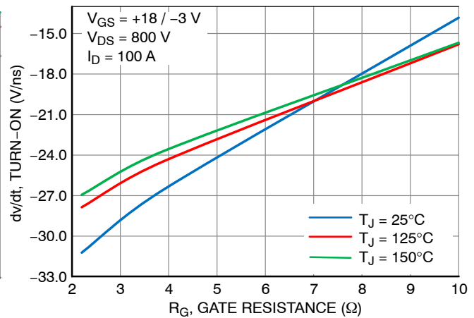
Figure 22. \frac{dv}{dt} Turn ON vs. Gate Resistance V_{DS} = 800 V
