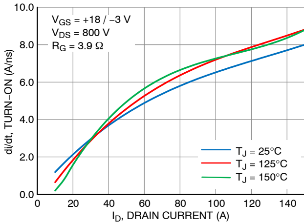
Figure 17. \frac{di}{dt} Turn ON vs. Drain Current V_{DS} = 800 V
