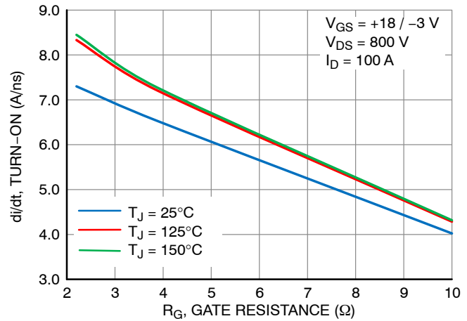
Figure 18. \frac{di}{dt} Turn ON vs. Gate Resistance V_{DS} = 800 V
