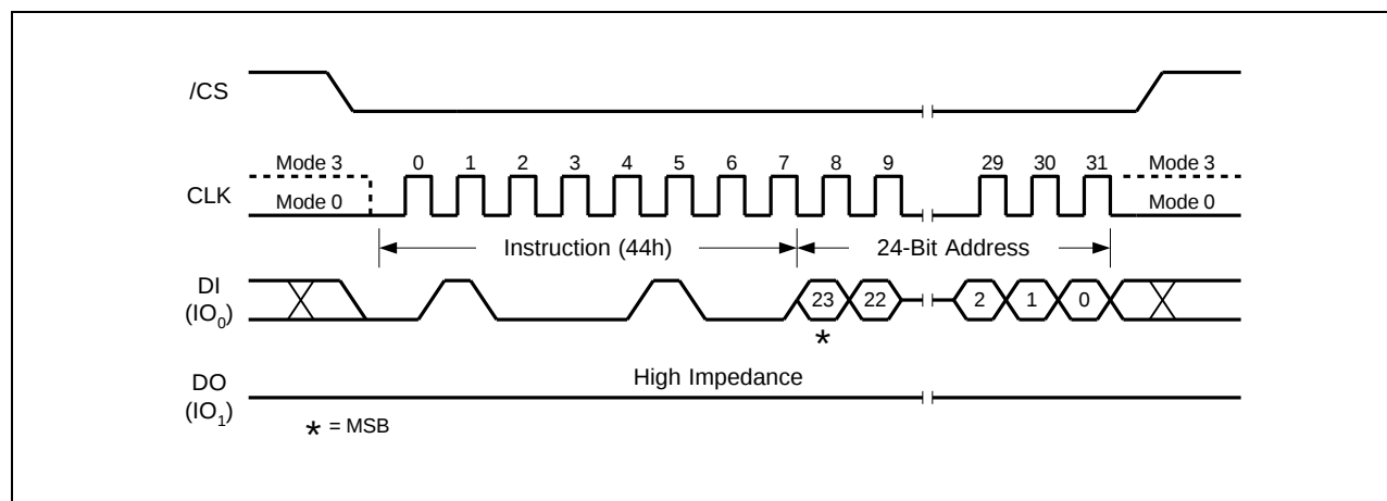
Figure 35. Erase Security Registers Instruction Sequence
