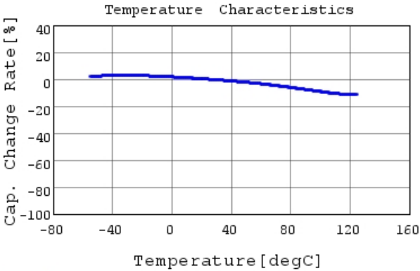
LLL216R71A224MA01 C-Temp. capchange, DC0.0V,
