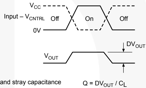
Figure 11. Charge Injection Test
