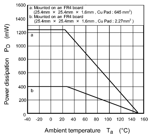
Fig. 8.11 P_D - T_a
