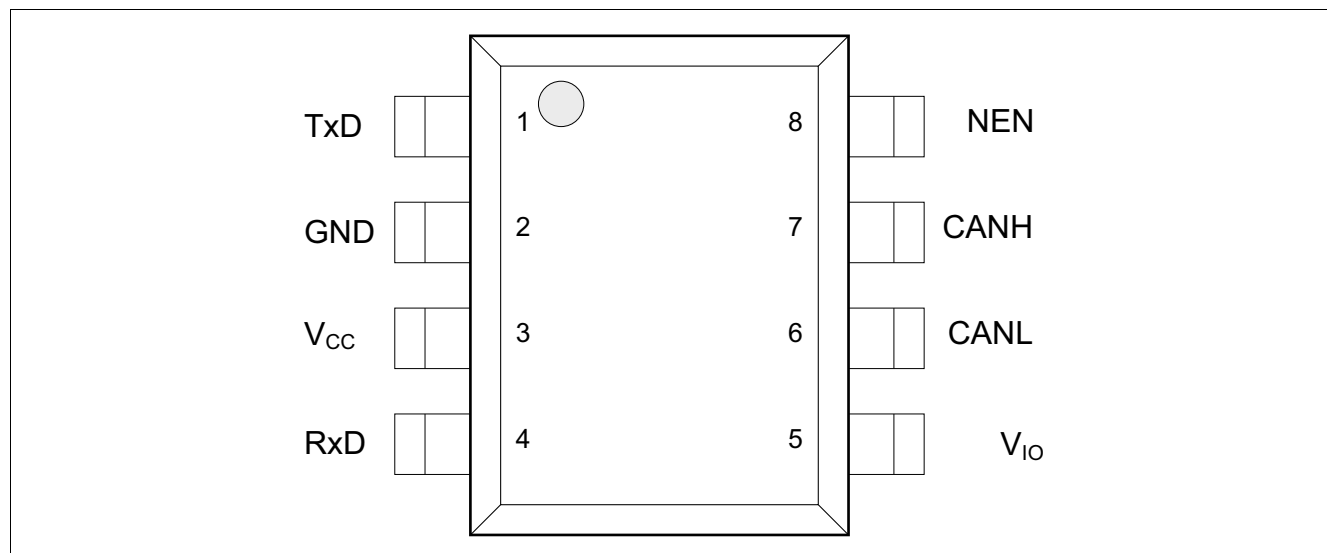
Figure 2 Pin configuration
