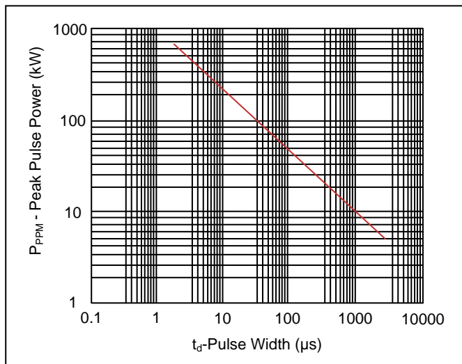
Figure 2. Peak Pulse Power Rating Curve
