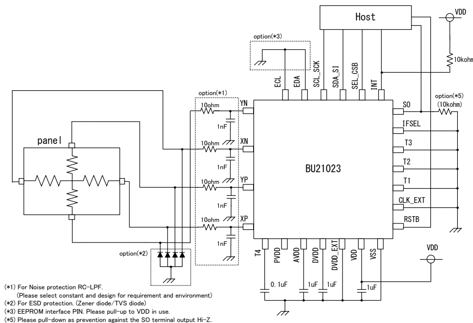
Example 1: BU21023GUL/MUV Application Circuit (4-wireSPI)
