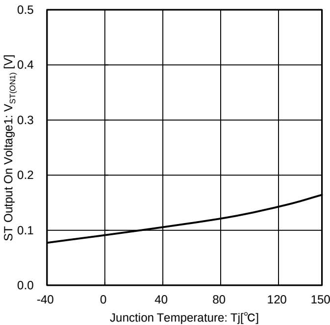
Figure 28. ST Output On Voltage1 vs Junction Temperature
