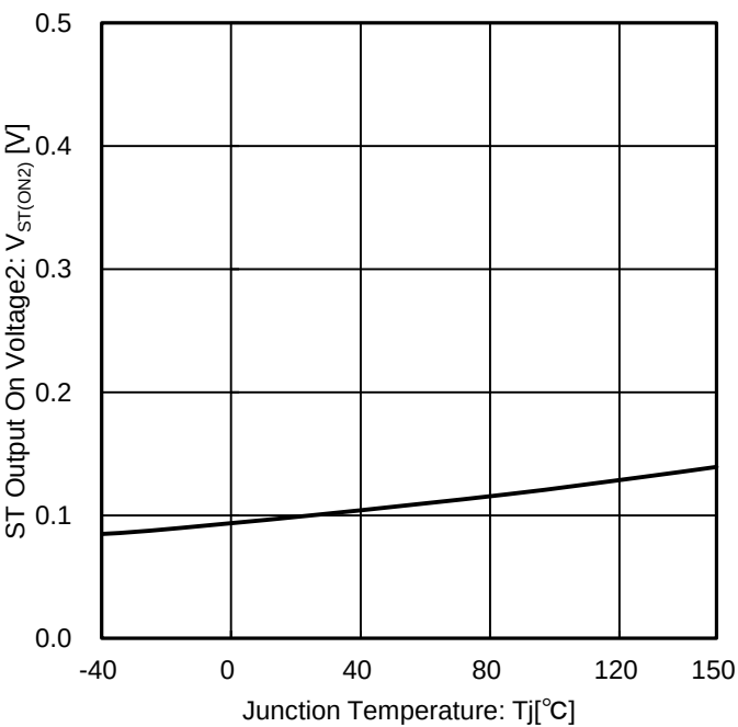
Figure 29. ST Output On Voltage2 vs Junction Temperature
