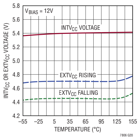
EXT CC Switchover and INTV CC Voltage vs Temperature
