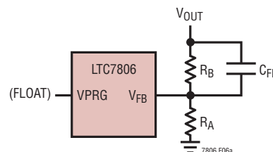
(a) Setting Boost Output Using External Resistors
