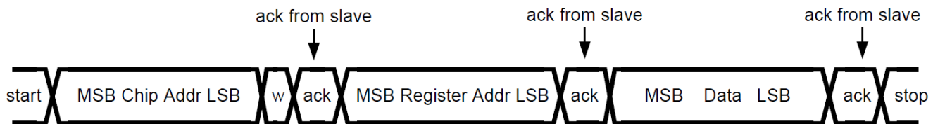
Figure 19. Write Cycle
