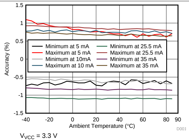
Figure 5. Channel-to-Channel Accuracy
