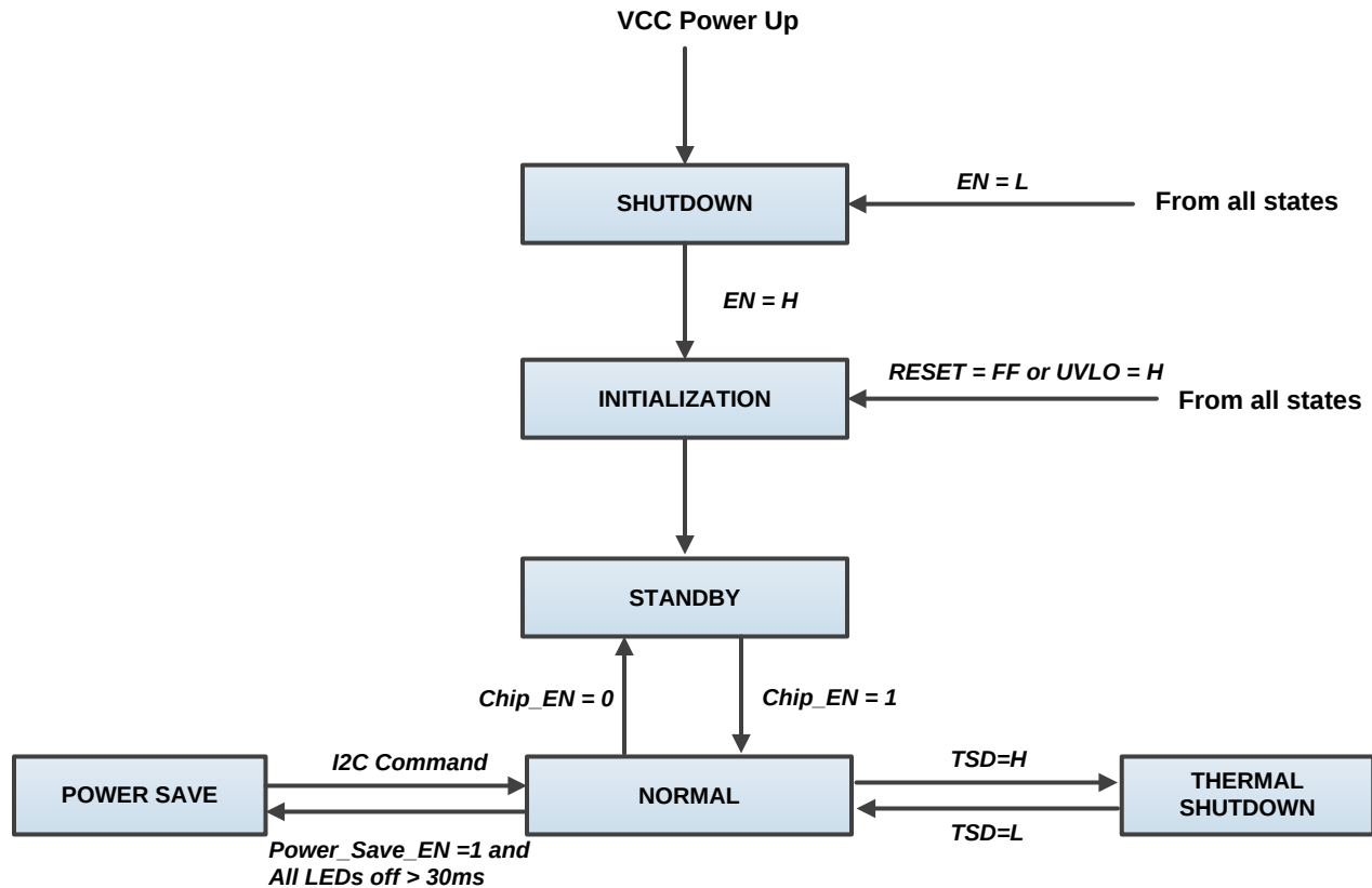
Figure 15. Functional Modes
