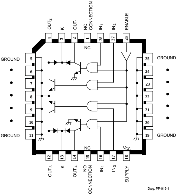
Package EB
