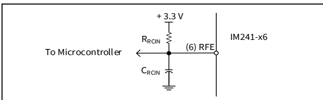
Figure 5 Typical PCB circuit connected to the RFE pin
