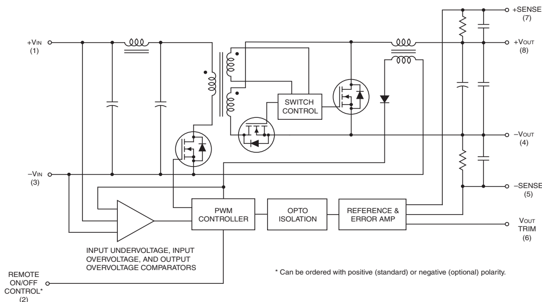
Figure 1. Simplified Schematic
