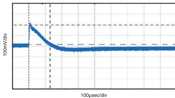
UCQ-3.3/30-D48 Output Transient Response ( V_{IN} = 48V , resistive load step 75% to 50%)
