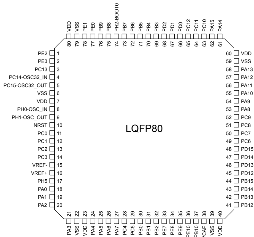
Figure 9. LQFP80 pinout
