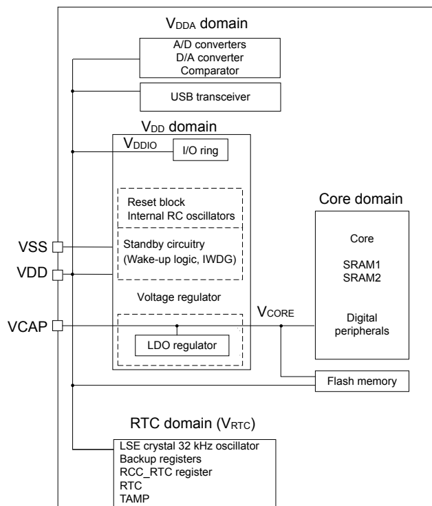
Figure 2. STM32C562xx power supply overview
