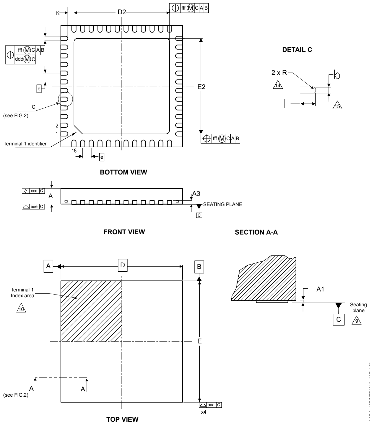
Figure 43. UFQFPN48 - Outline
