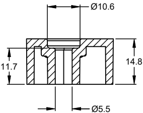
SECTION B-B FOR #10 THRU BOLT 2X
