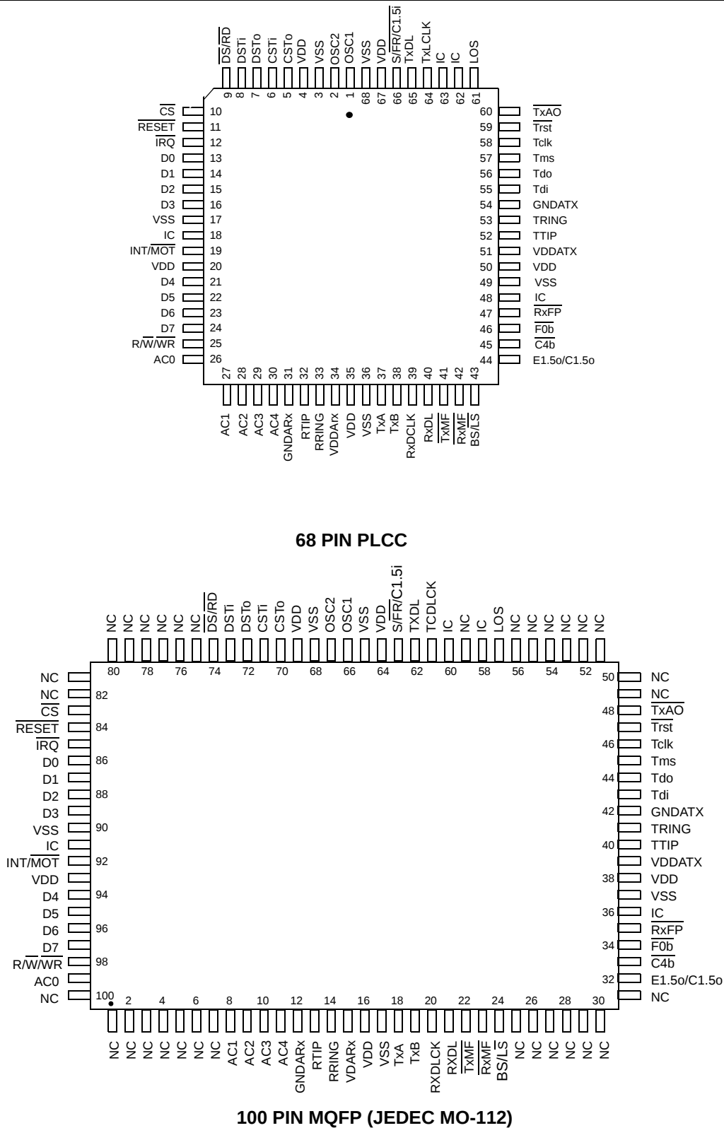
Figure 2 - Pin Connections
