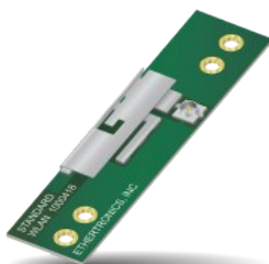
1000418 – WLAN / Bluetooth / Zigbee Embedded Stamped Metal Antenna
