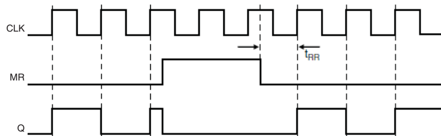
FIGURE 1. TIMING DIAGRAM
