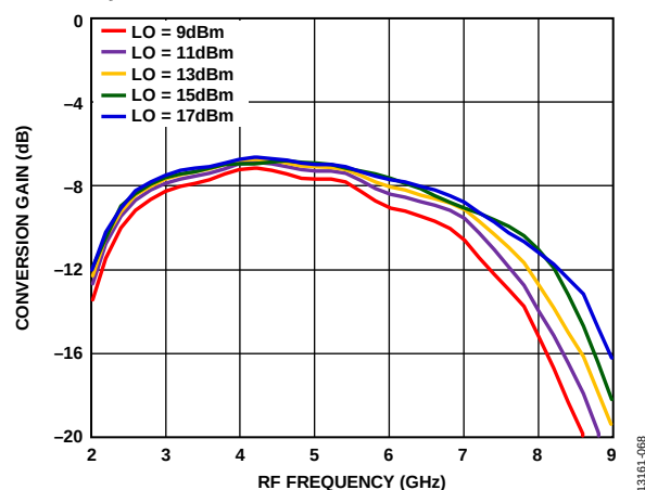
Figure 76. Conversion Gain vs. RF Frequency at Various LO Drives
