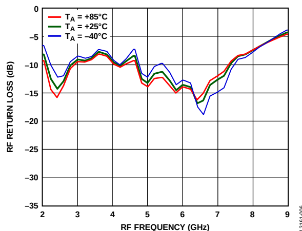
Figure 12. RF Port Return Loss vs. RF Frequency, LO Frequency = 4.6 GHz, LO Drive = 15 dBm
