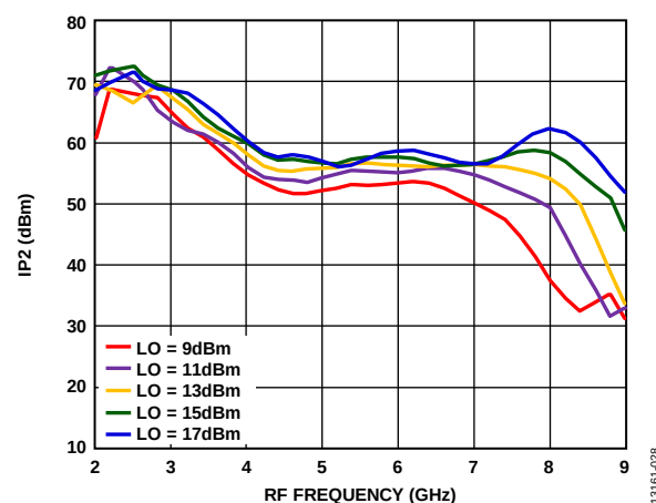
Figure 34. Input IP2 vs. RF Frequency at Various LO Drives
