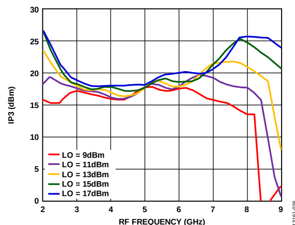
Figure 33. Input IP3 vs. RF Frequency at Various LO Drives
