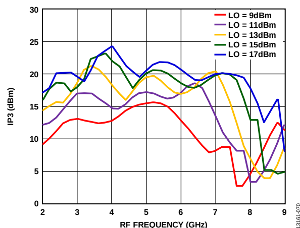
Figure 77. Input IP3 vs. RF Frequency at Various LO Drives
