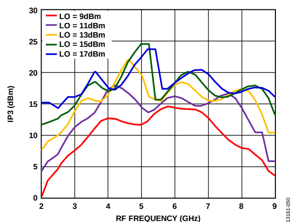
Figure 57. Input IP3 vs. RF Frequency at Various LO Drives
