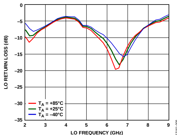
Figure 11. LO Port Return Loss vs. LO Frequency, LO Drive = 15 dBm
