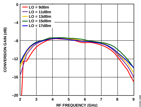
Figure 56. Conversion Gain vs. RF Frequency at Various LO Drives
