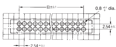
Standard terminal arrangement
