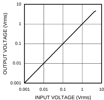
Fig.12 Output Voltage - Input Voltage (BD3811K1)
