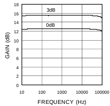
Fig.22 Center Mixing - Frequency (BD3818KS)
