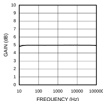
Fig.11 Voltage Gain - Frequency LINE (BD3818KS)
