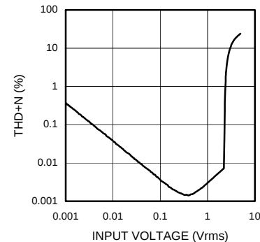
Fig.15 THD+N - Input Voltage LINE (BD3818KS)
