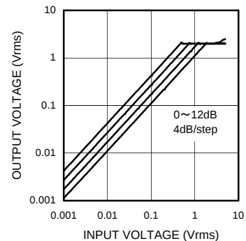
Fig.25 AGC Output Voltage - Input Voltage (BD3818KS)
