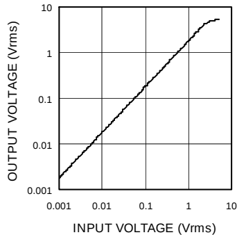
Fig.13 Output Voltage - Input Voltage LINE (BD3818KS)
