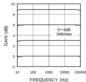
Fig.17 Input Gain - Frequency (BD3818KS)
