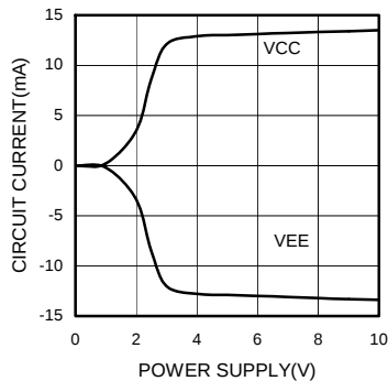
Fig.8 Circuit Current - Power Supply (BD3811K1)
