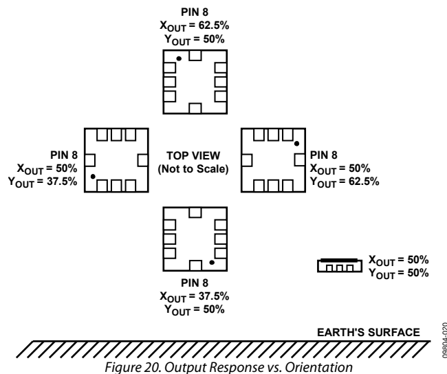
Figure 20. Output Response vs. Orientation
