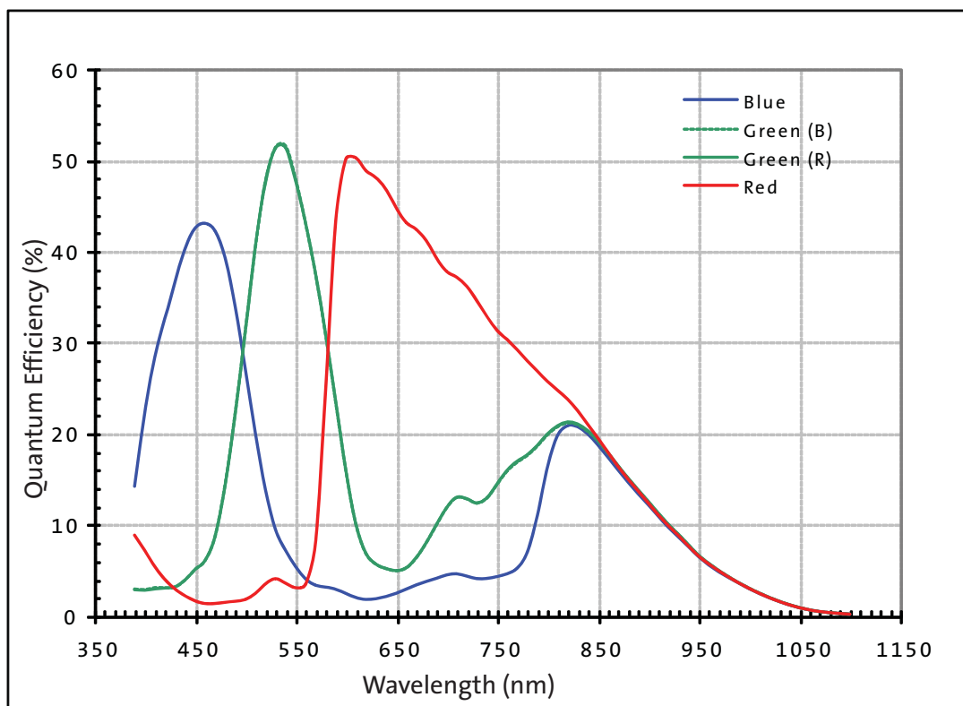
Figure 56: Quantum Efficiency
