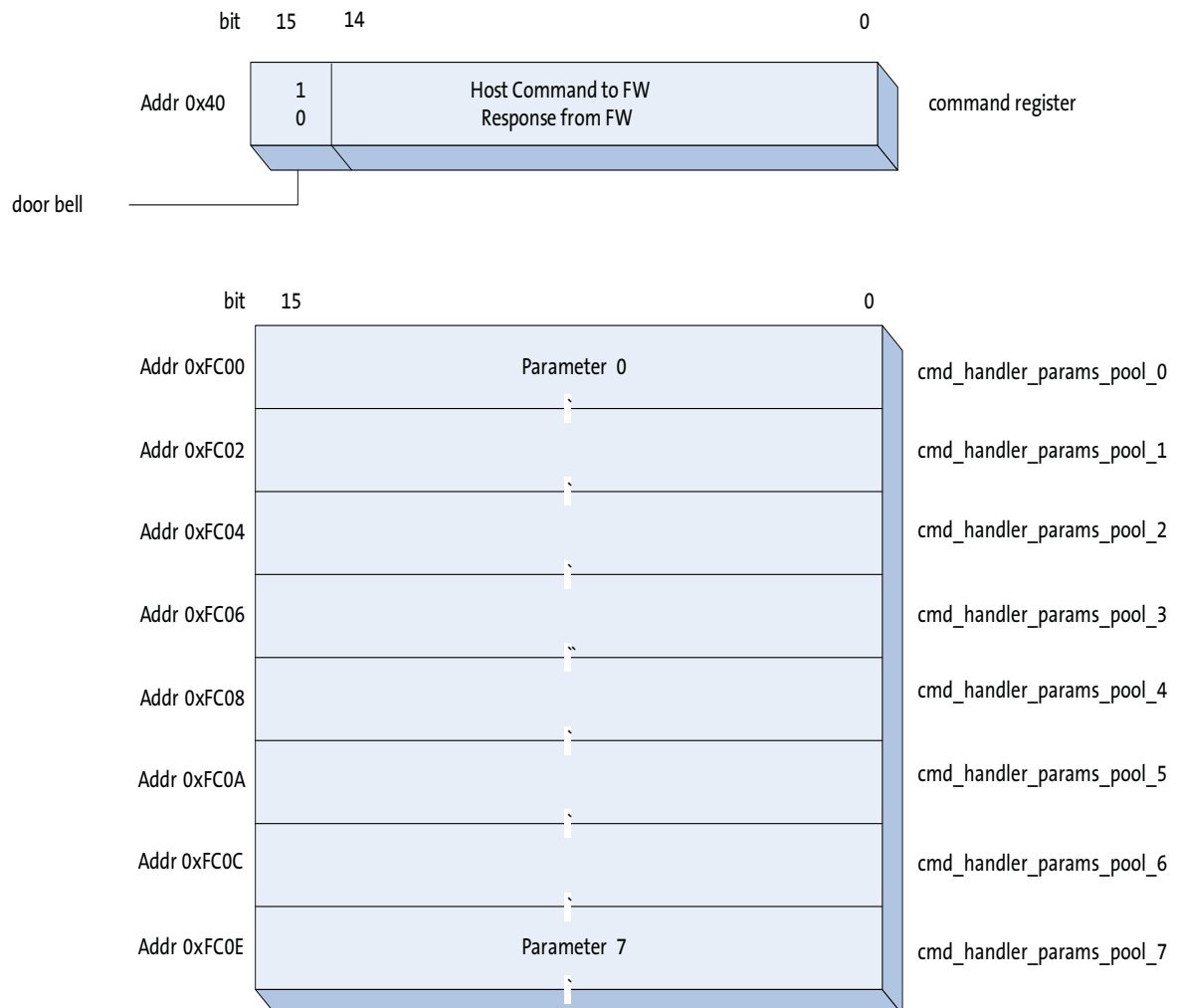
Figure 21: Interface Structure
