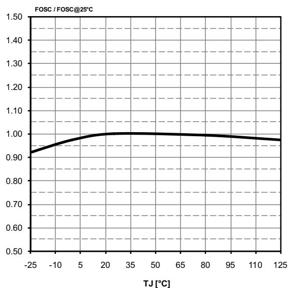
Figure 8. Switching frequency vs. T_J
