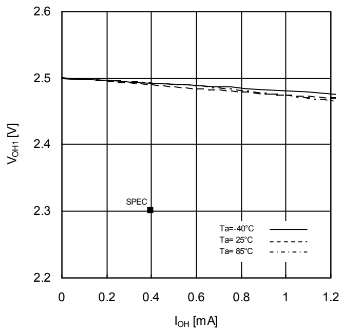
Figure 9. Output High Voltage1 vs Output Current ( V_{CC} = 2.5V )
