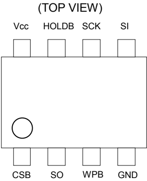
Figure 4. Pin Configuration
