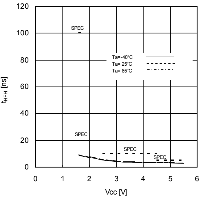
Figure 30. HOLDB Setting Hold Time vs Supply Voltage
