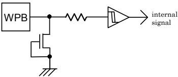
Figure 51. WPB input equivalent circuit
