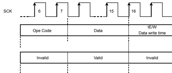
Figure 37. WPB valid timing (At inputting WRSR command)
