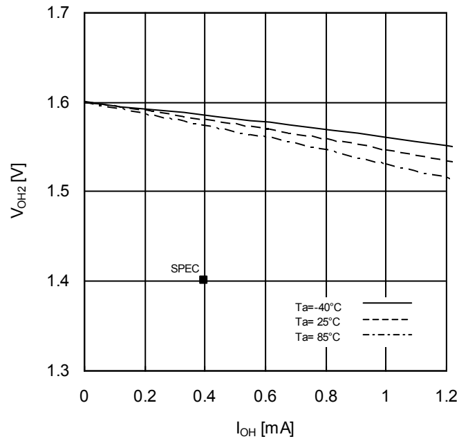
Figure 10. Output High Voltage2 vs Output Current ( V_{CC} = 1.6V )
