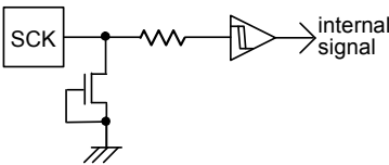
Figure 48. SCK input equivalent circuit
