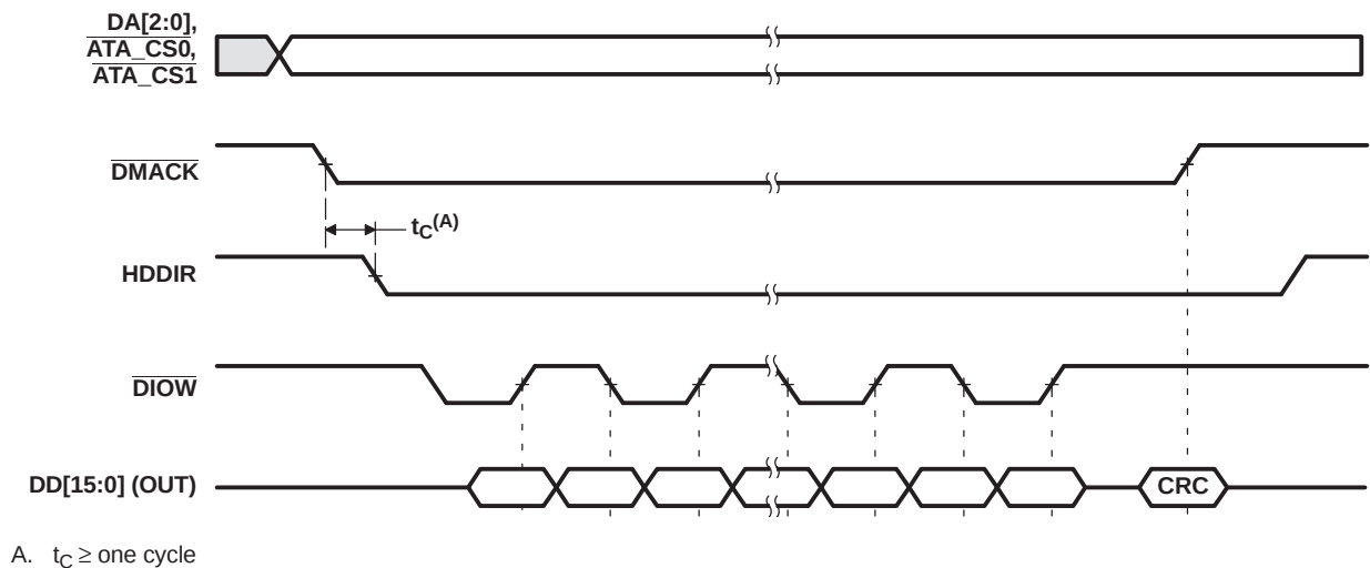
Figure 7-80. ATA HDDIR Ultra DMA Write Transfer Timing
