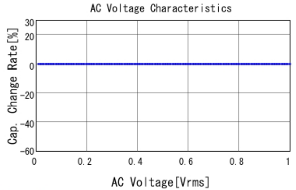
ECASD60E477M009K00 C-AC Voltage capchange, DC0V, 2
