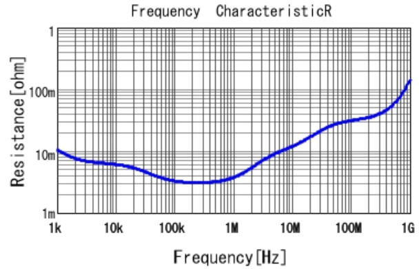
ECASD60E477M009K00 R DC0V, 25degC
