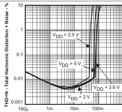
Figure 4. Total Harmonic Distortion + Noise vs Output Power
