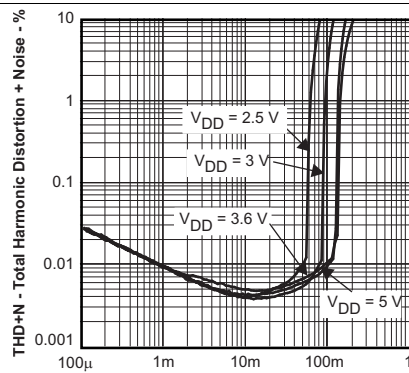
Figure 3. Total Harmonic Distortion + Noise vs Output Power
