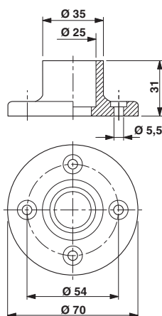
Dimensional drawing
