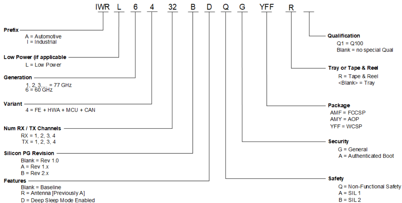
Figure 10-1. Device Nomenclature
