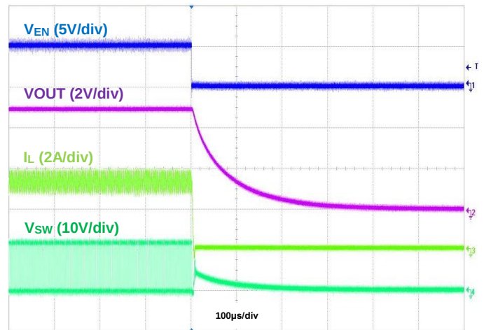
Figure 20. Shutdown Using EN, IOU = 3.5A
