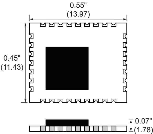
Figure 18: HumPRO™ Series Transceiver Dimensions
