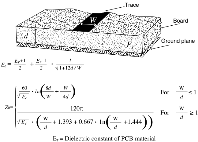
Figure 115: Microstrip Formulas
