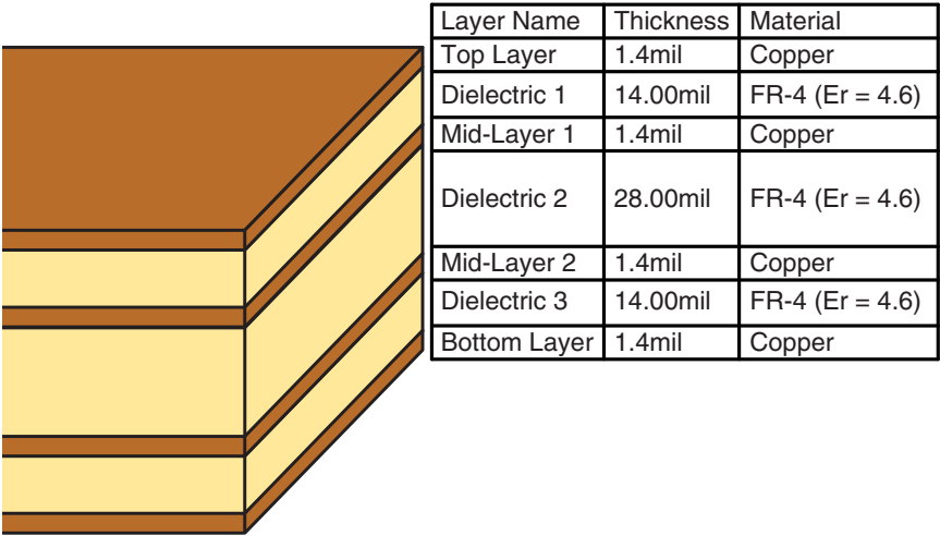
Figure 109: HumPRO™ Series Transceiver Castellation Version Reference Design PCB Stack
