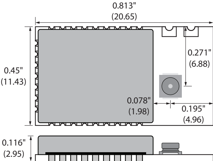
Figure 19: HumPRO™ Series Transceiver Pre-certified Version Dimensions
