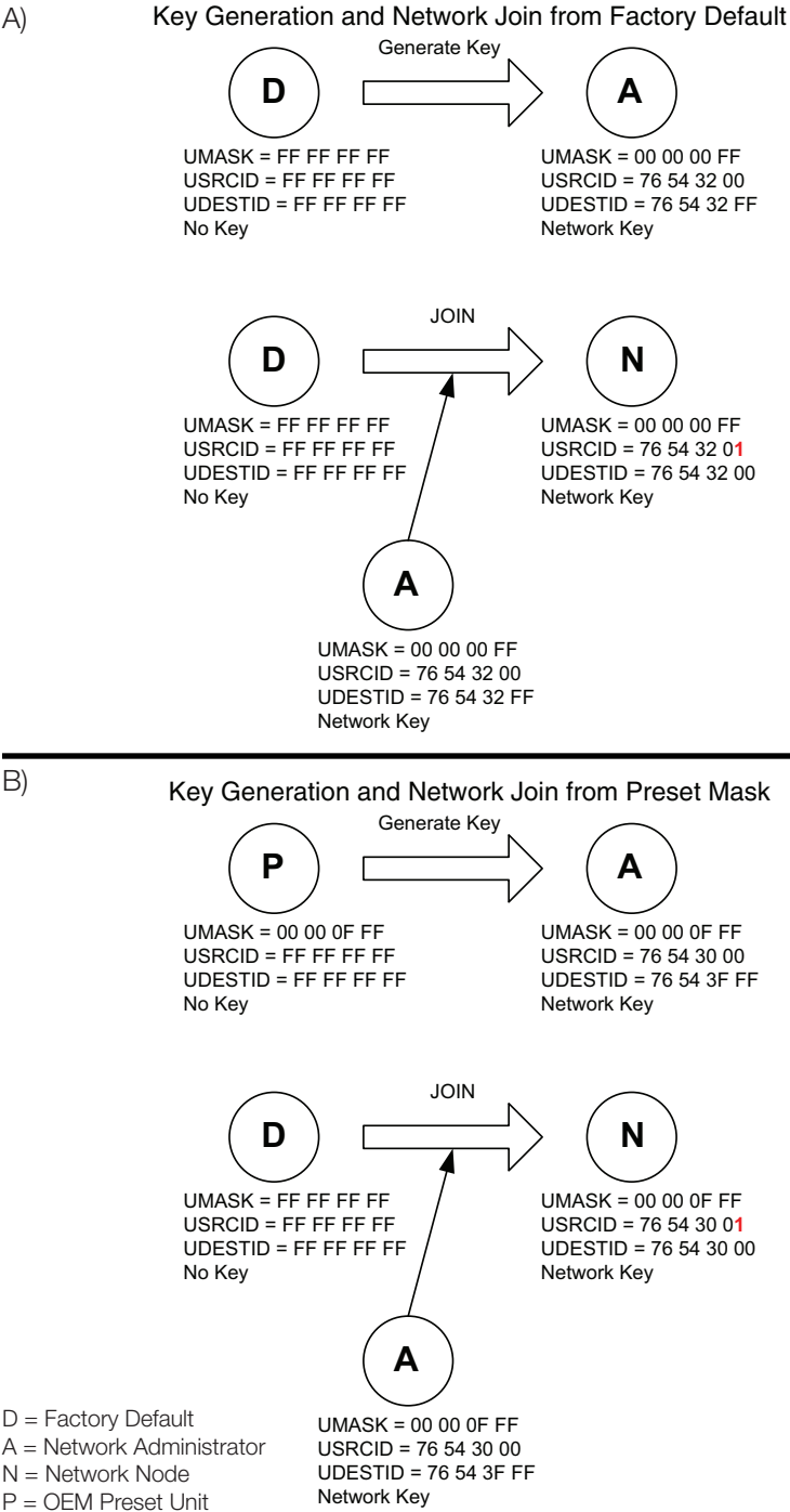
Figure 31: HumPRO™ Series JOIN Process
