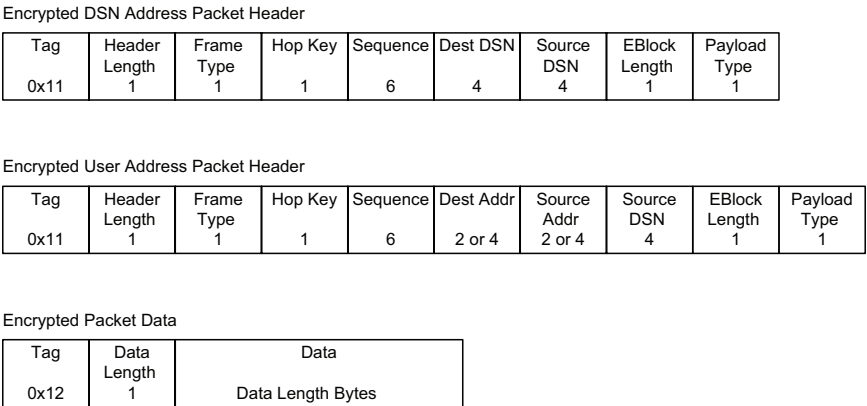
Figure 25: HumPRO™ Series Transceiver Encrypted Packet Header and Data Structure
