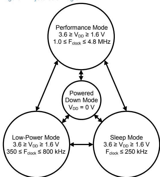
Figure 3: State Diagram
