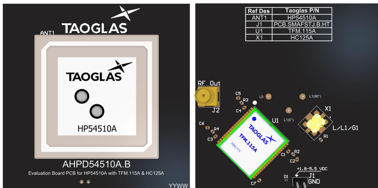
Top and bottom view of PCB.
