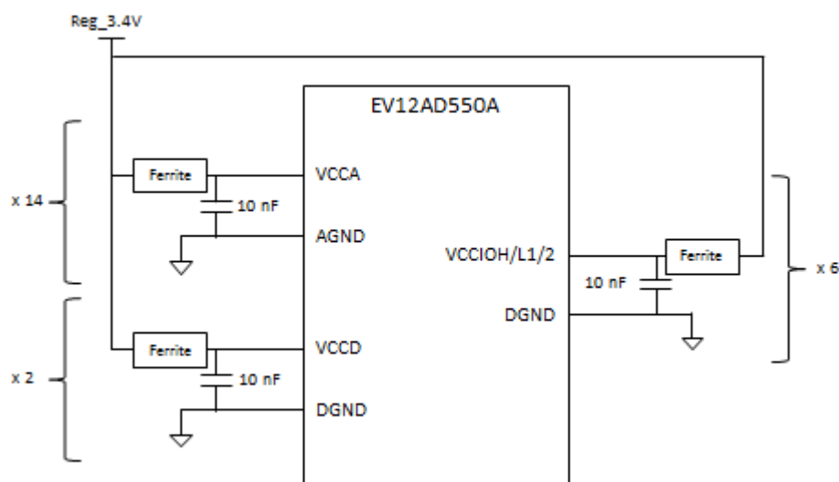
Figure 28: Decoupling with single supply at 3.4V
