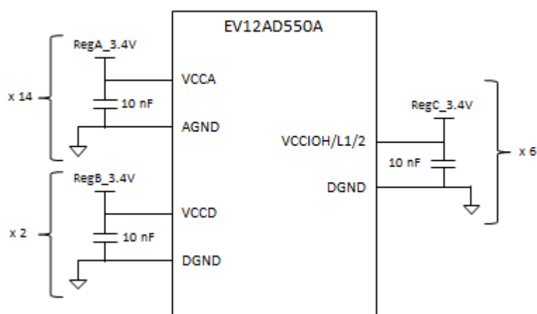
Figure 27: Decoupling with separate supplies
