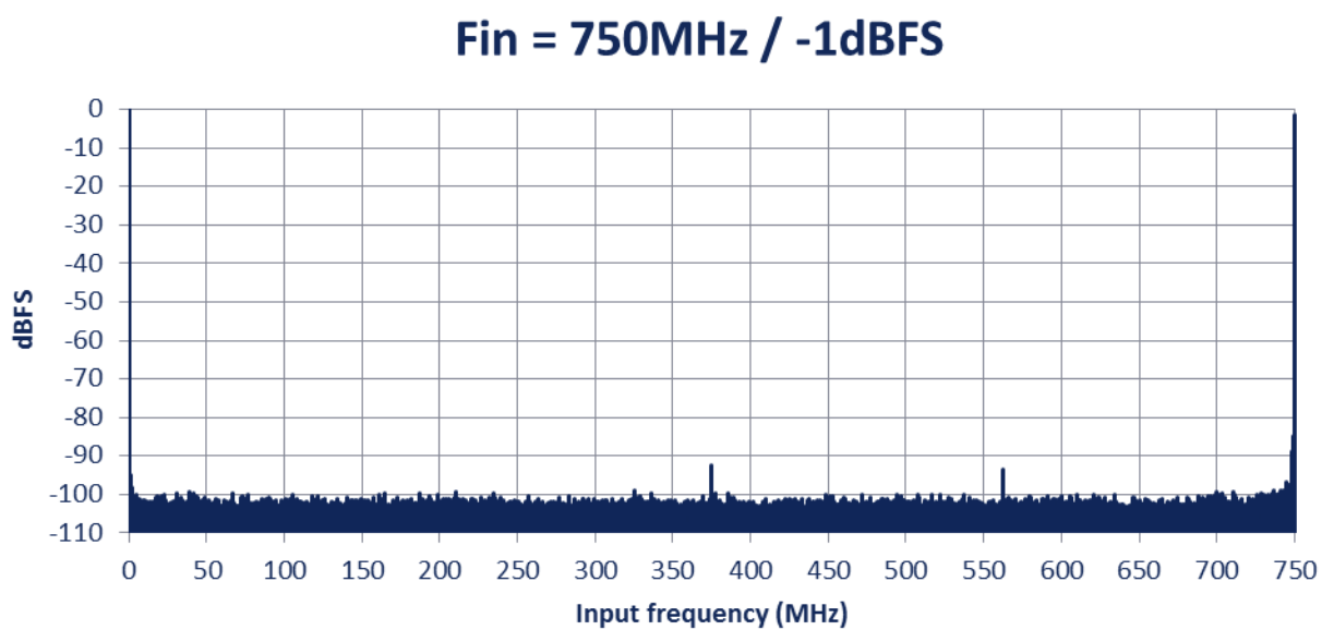
Figure 26: Spectral purity at F_s=1.5\text{GSps} and F_{in} = 750\text{MHz} / -1\text{dBFS}
