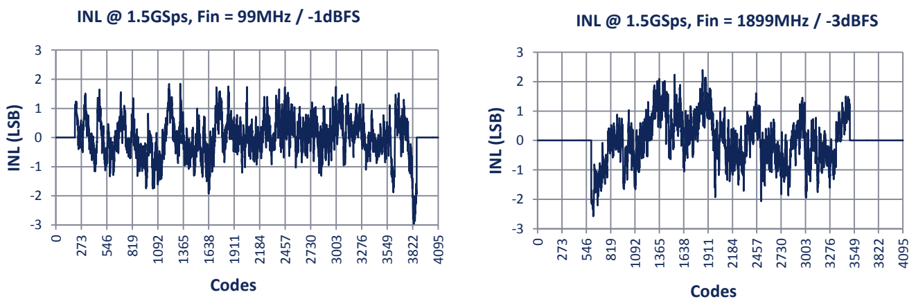
Figure 22: INL performances at F_{\text{clock}} = 3\text{GHz} ( F_s = 1.5\text{GSps} )
