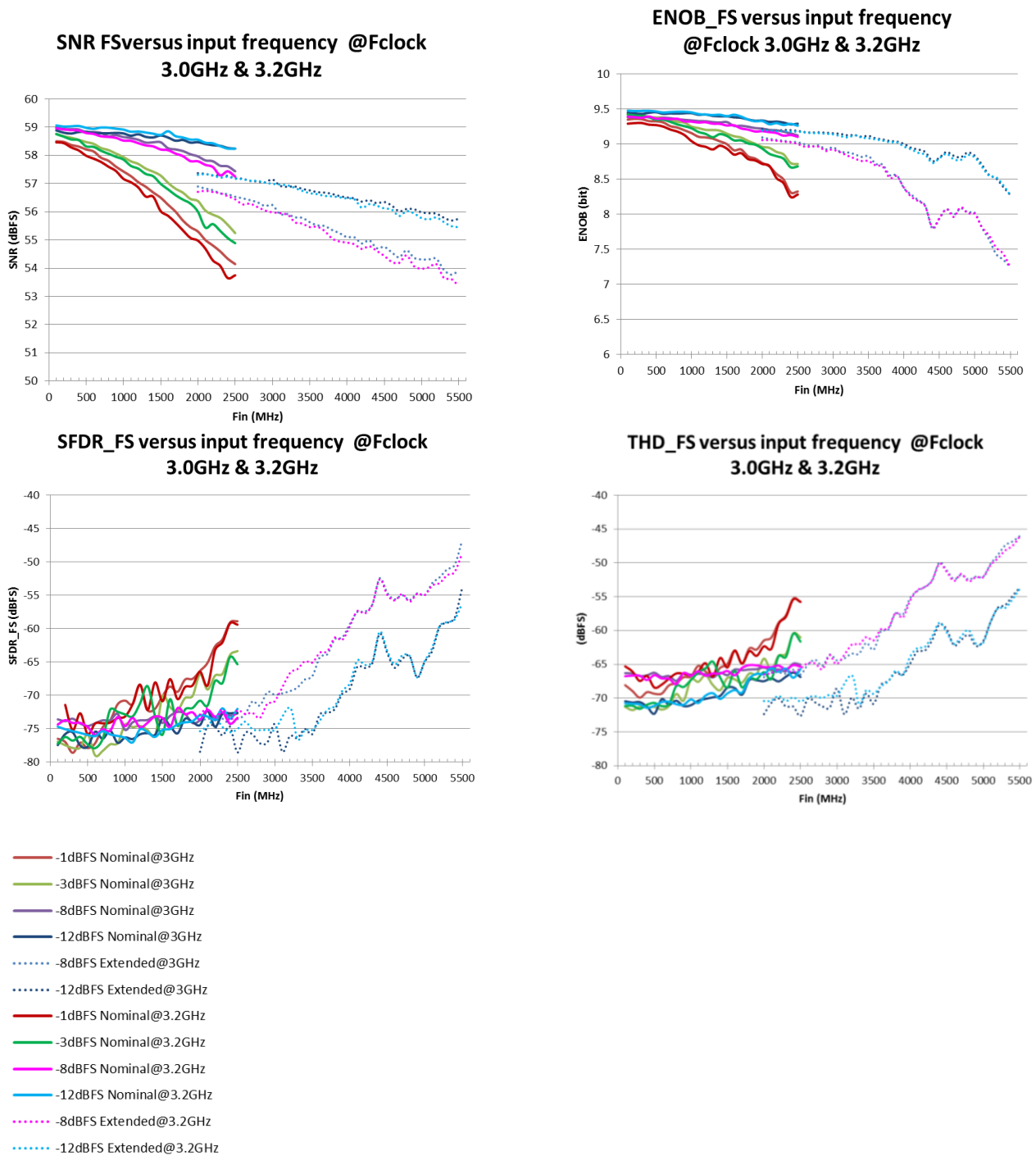
Figure 23: FFT performances vs input frequency in typical conditions @ Fclock = 3GHz & Fclock = 3.2GHz
