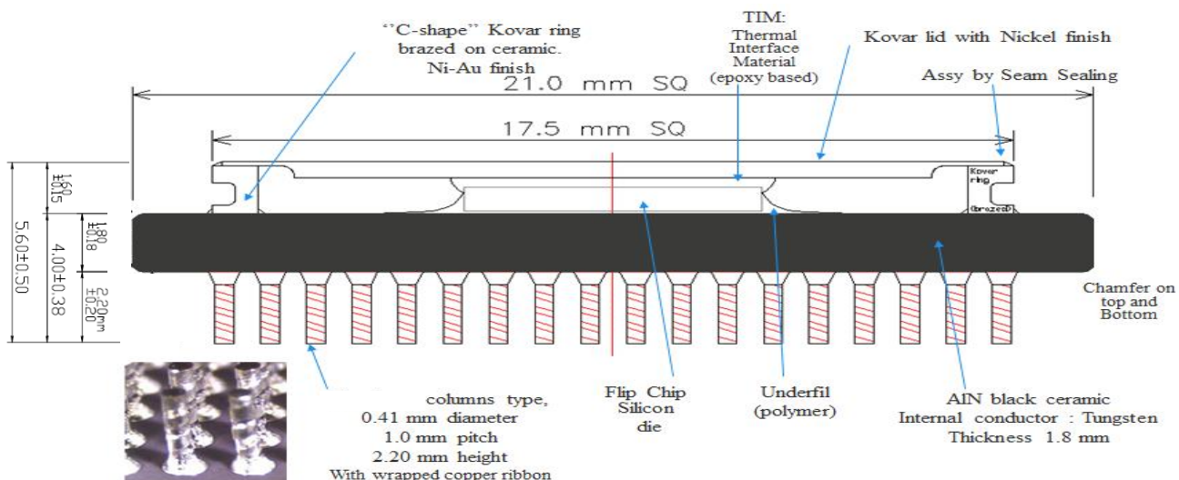
Figure 9: Package cross-section
