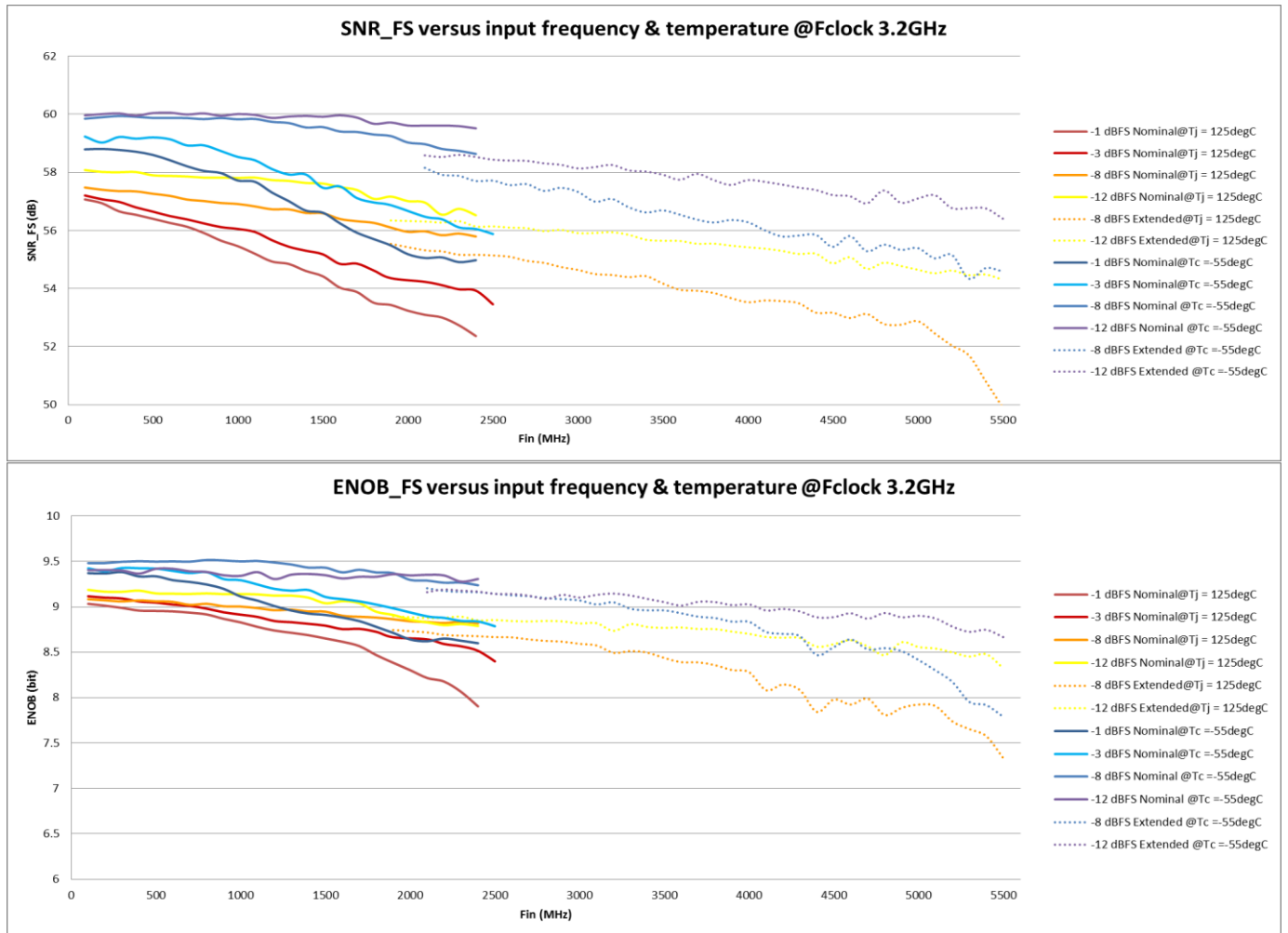
Figure 24: FFT performances vs temperature @ Fclock = 3.2GHz
