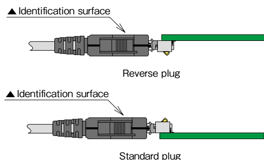
Plug variations
