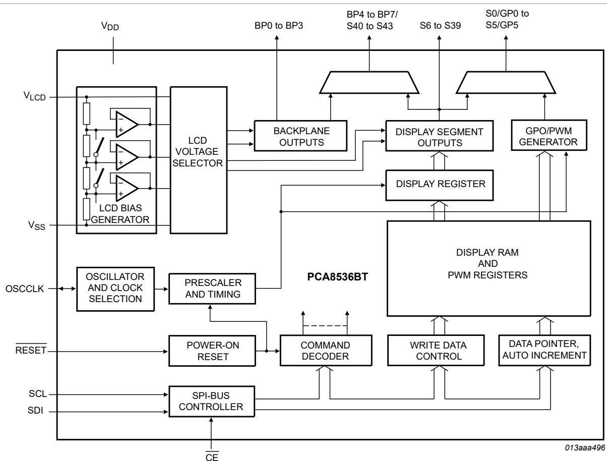
Figure 2. Block diagram of PCA8536BT
