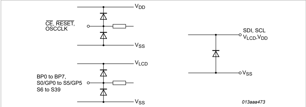
Figure 42. Device protection diagram for PCA8536BT
