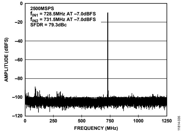
Figure 42. Two Tone FFT Plot at 2.5 GSPS, f_{IN1} = 728.5 MHz and f_{IN2} = 731.5 MHz at AIN, -7.0 dBFS (SFDR = 79.3 dBc)
