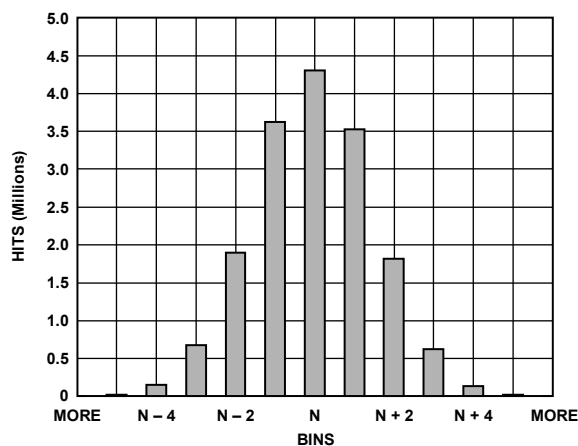
Figure 18. Input Referred Noise Histogram with 2.0 GSPS
