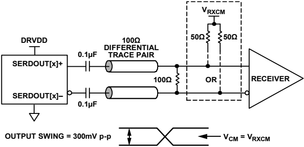
Figure 89. AC-Coupled Digital Output Termination Example
